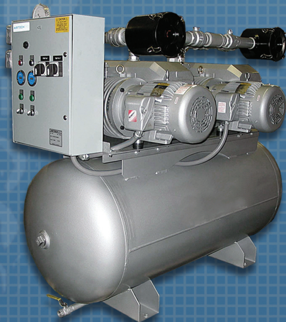
DUPLEX HORIZONTAL TANK MOUNTED ROTARY VANE VACUUM PACKAGE
